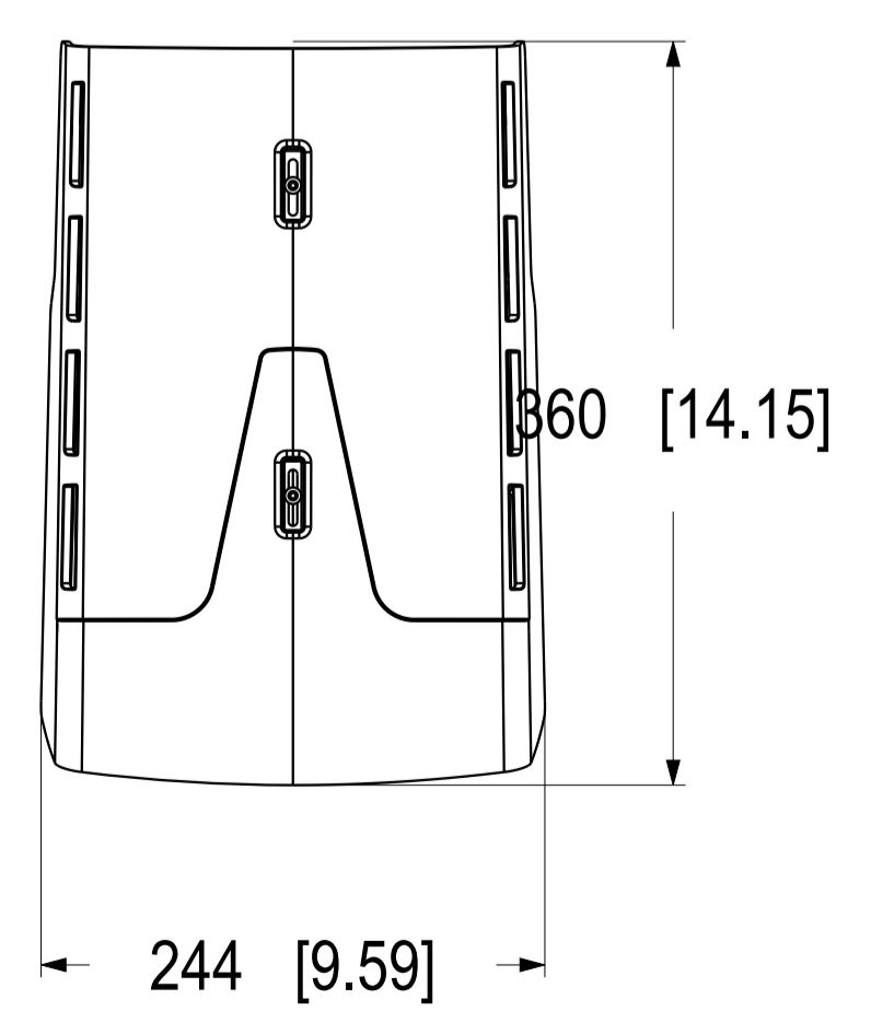
AXIS Q8752-E MkII Bispectral PTZ Camera
