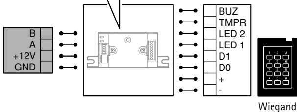
AXIS TA1101-B Wiegand to OSDP Converter
